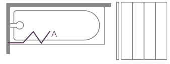
A: Moving Panels (screen width when folded into the bath 228mm) Recommended shower head position
